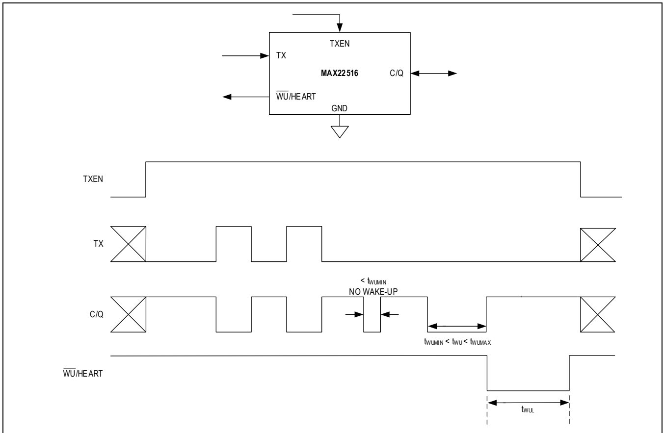
Figure 5. Wake-Up Detection
