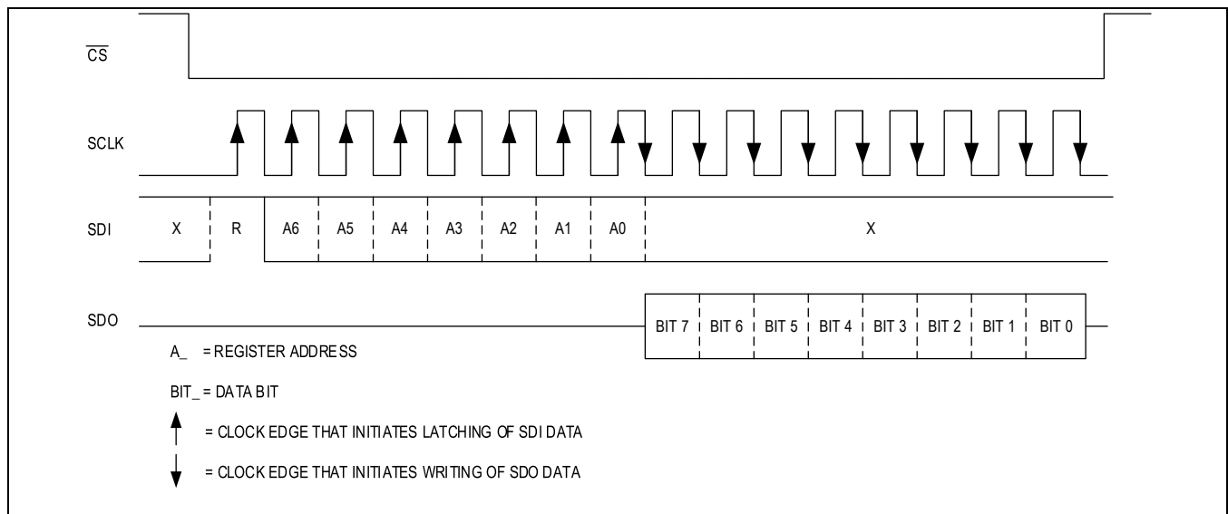
Figure 10. SPI Read Byte
