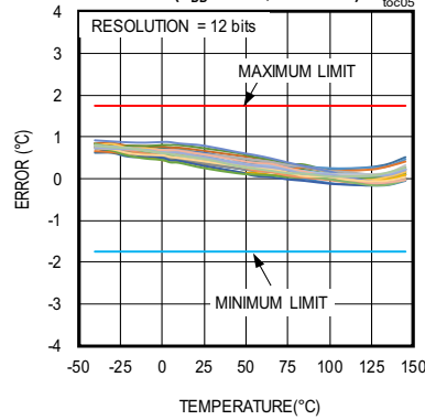
ACCURACY vs. TEMPERATURE ( V_{DD} = 1.6\text{V} , 30 UNITS)
