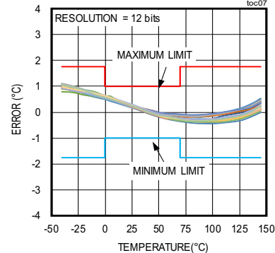
ACCURACY vs. TEMPERATURE ( V_{DD} = 3.3\text{V} , 30 UNITS)
