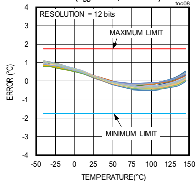
ACCURACY vs. TEMPERATURE ( V_{DD} = 3.6\text{V} , 30 UNITS)
