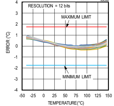
ACCURACY vs. TEMPERATURE ( V_{DD} = 2.5\text{V} , 30 UNITS)
