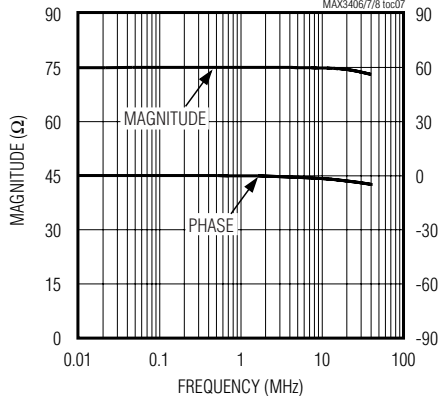
IMPEDANCE vs. FREQUENCY 75Ω MODE—MAX3406/MAX3407
