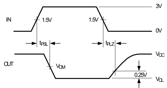
Figure 6. Driver Enable and Disable Times ( t_{PZL} , t_{PSL} , t_{PLZ} )
