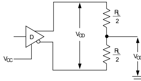
Figure 2. Driver V_{OD} and V_{OC}
