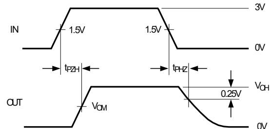
Figure 5. Driver Enable and Disable Times ( t_{PZH} , t_{PSH} , t_{PHZ} )
