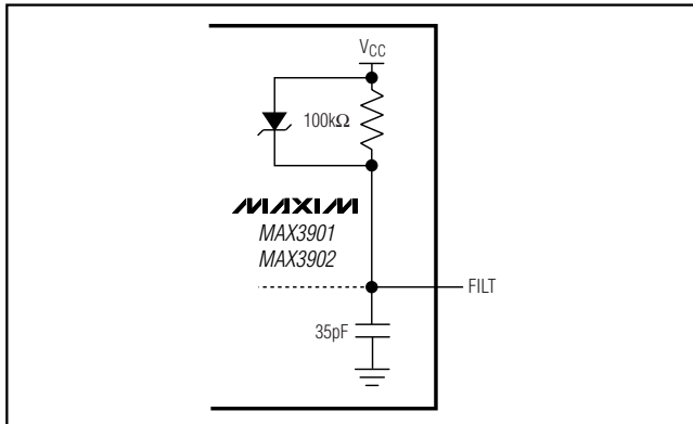
Figure 5. FILT pad
