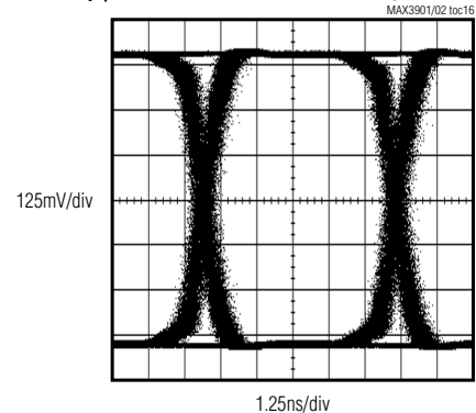
OUTPUT EYE DIAGRAM (2 \mu A -p-p ELECTRICAL INPUT AT T_J = +140^\circ C )
