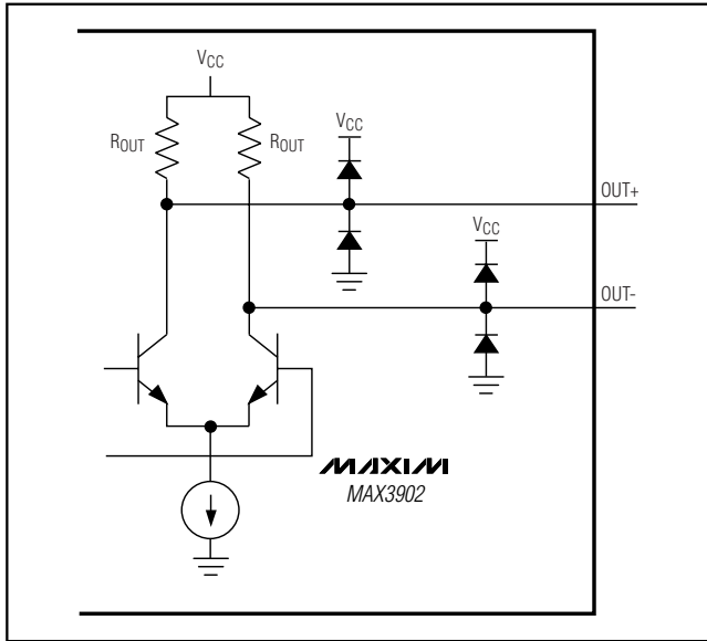
Figure 3. MAX3902 CML Output
