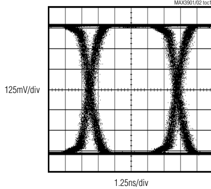
OUTPUT EYE DIAGRAM (2 \mu A -p-p ELECTRICAL INPUT AT T_J = -40^\circ C )
