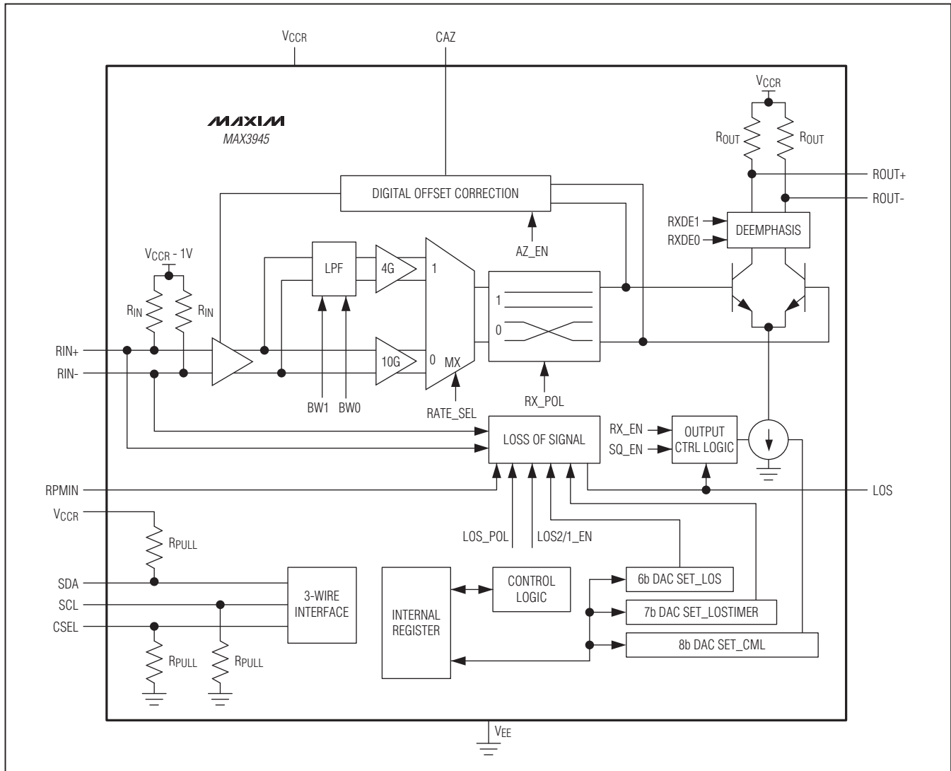
Figure 2. Functional Diagram
