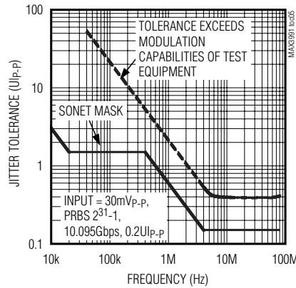
JITTER TOLERANCE vs. FREQUENCY
