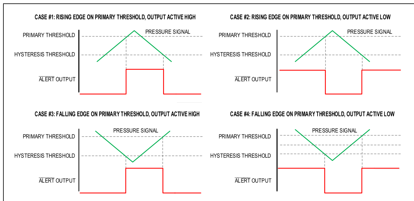
Figure 2. \overline{\text{ALERT}} Cases
