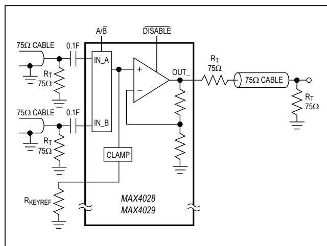
Figure 3. Video Line Driver
