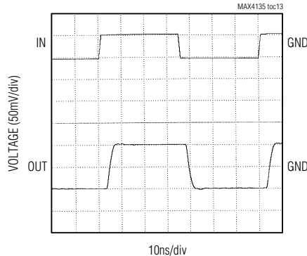
MAX4136 SMALL-SIGNAL PULSE RESPONSE ( A_{VCL} = 2 )
