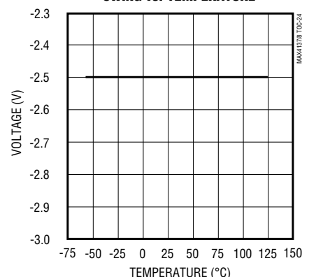
NEGATIVE OUTPUT VOLTAGE SWING vs. TEMPERATURE
