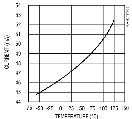
POWER SUPPLY CURRENT vs. TEMPERATURE
