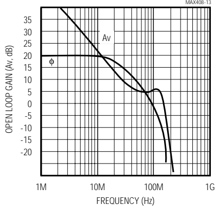
OPEN LOOP FREQUENCY RESPONSE, R L = 2kΩ, C L = 50pF
