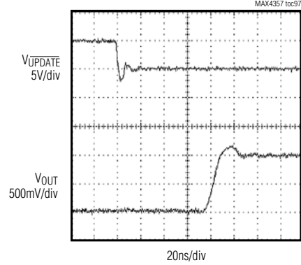
SWITCHING TIME
