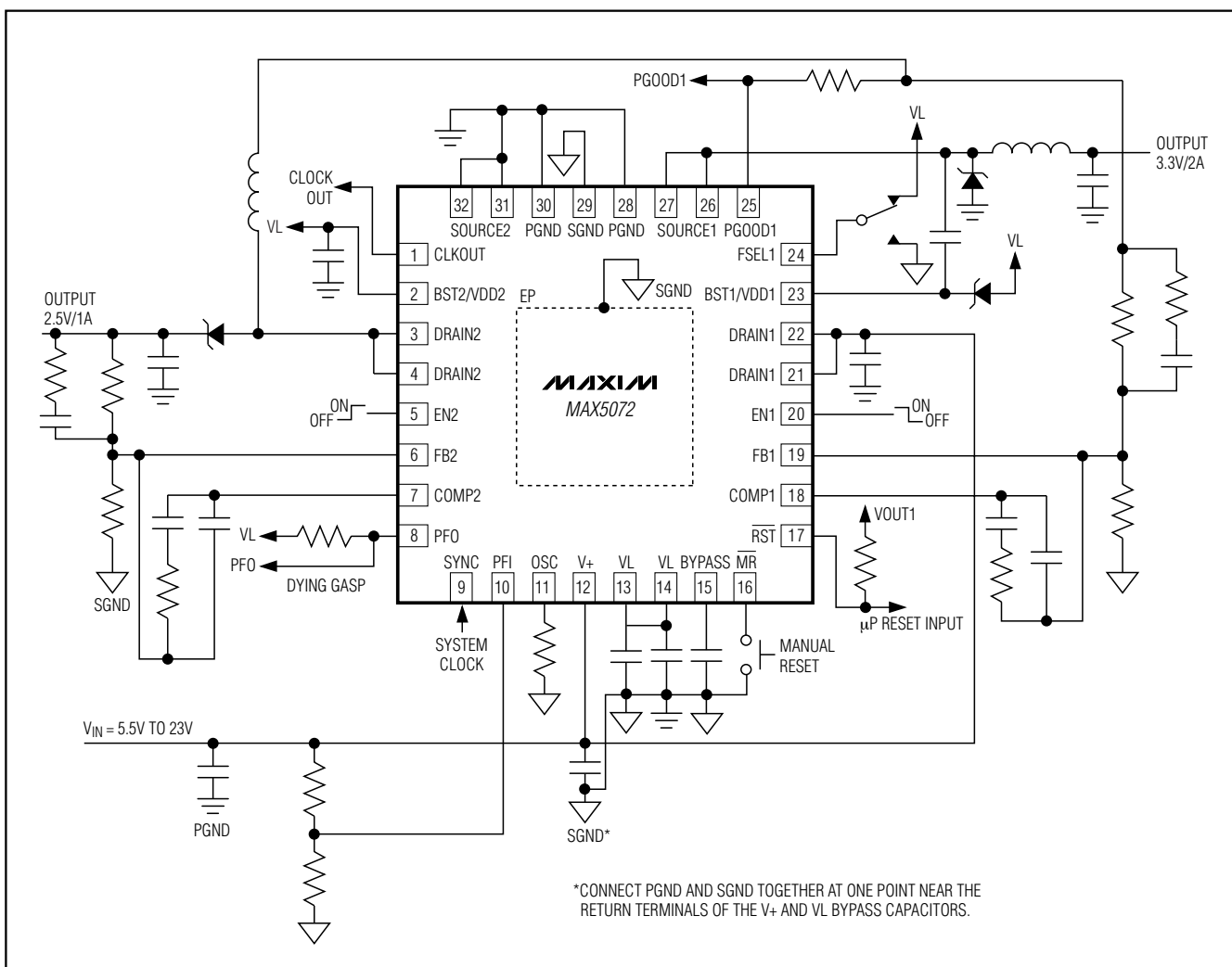
Figure 9. Buck-Boost Application
