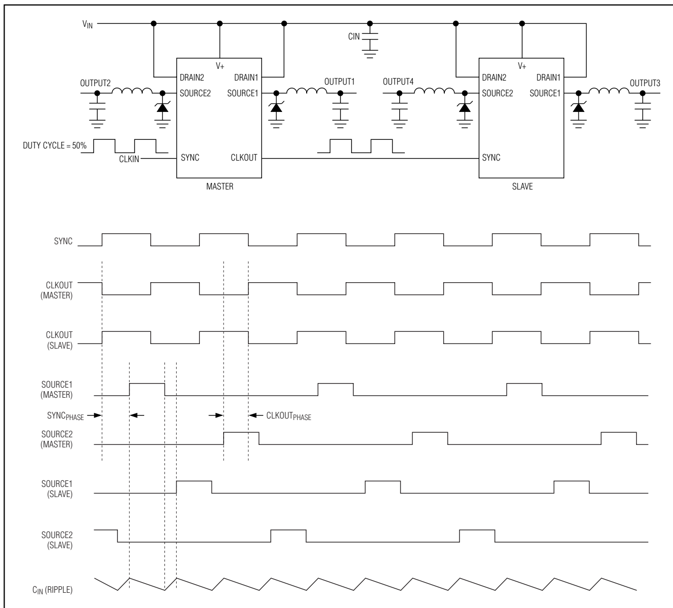
Figure 3. Synchronized Controllers
