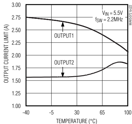
OUTPUT LOAD CURRENT LIMIT vs. TEMPERATURE
