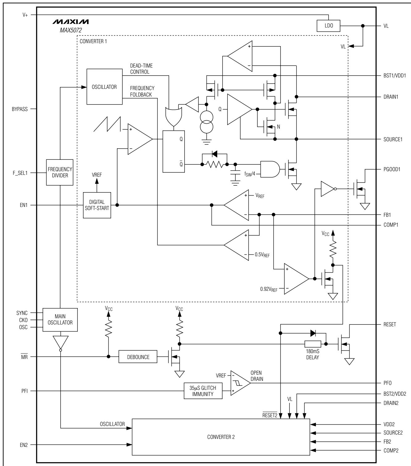
Figure 2. Functional Diagram
