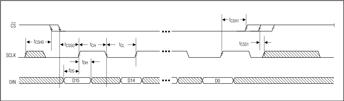
Figure 1. Timing Diagram
