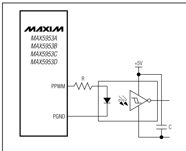
Figure 5. Secondary-Side Synchronous Rectifier Driver Using a High-Speed Optocoupler
