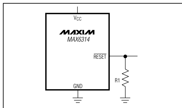
Figure 3. \overline{\text{RESET}} Valid to V_{CC} = \text{Ground} Circuit
