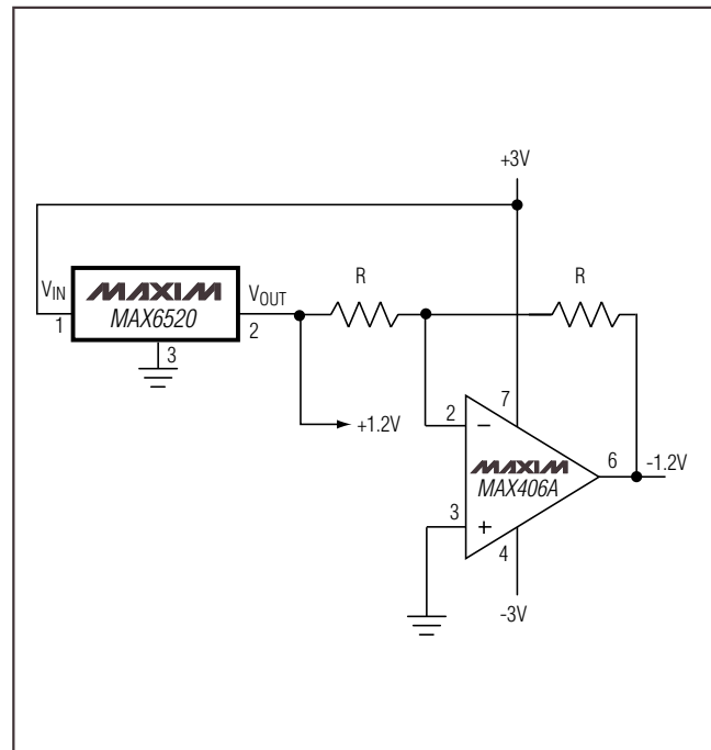
Figure 2. Low-Power \pm 1.2V Reference
