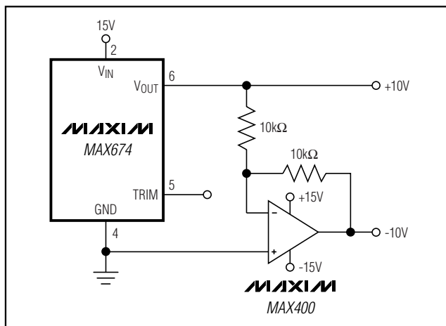
Figure 3. \pm 10V Reference
