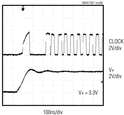
SETTLING TIME FROM START
