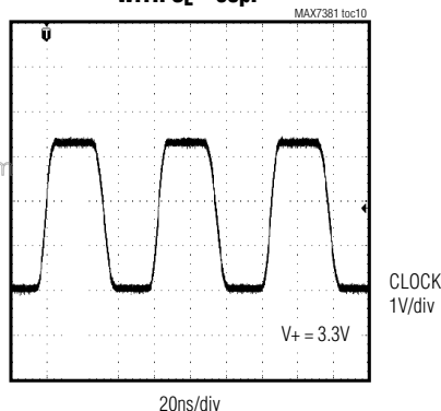
CLOCK OUTPUT WAVEFORM WITH C_L = 50pF
