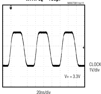
CLOCK OUTPUT WAVEFORM WITH C_L = 100pF
