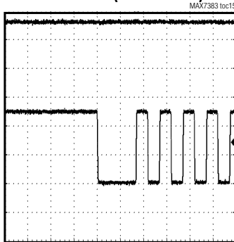
LOW-SPEED TO HIGH-SPEED TRANSITION (DETAIL ZOOM)
