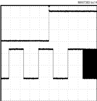
LOW-SPEED TO HIGH-SPEED TRANSITION
