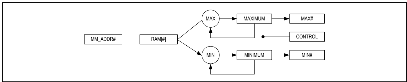
Figure 13. Min/Max Tracking
