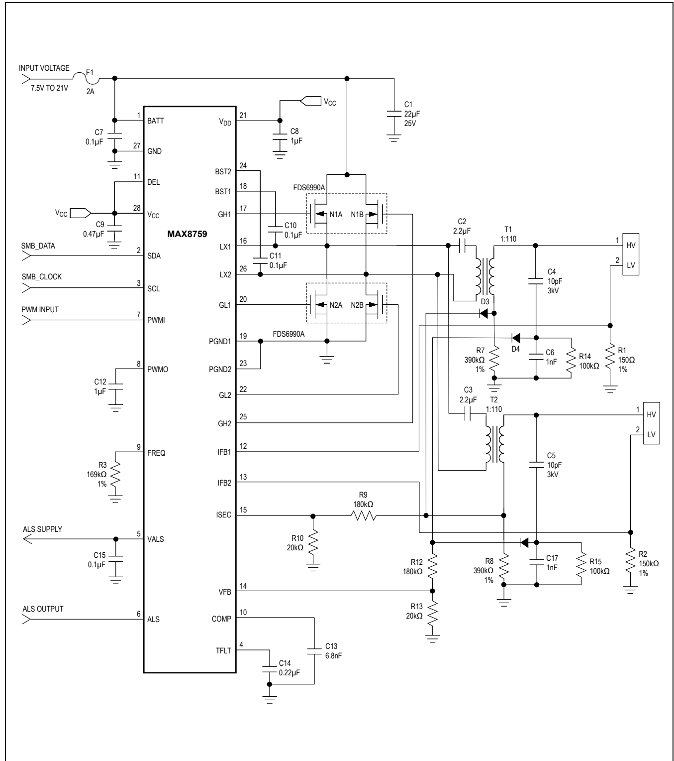
Figure 11. Typical MAX8759 Dual-Lamp Operating Circuit
