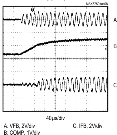
DPWM SOFT-START
