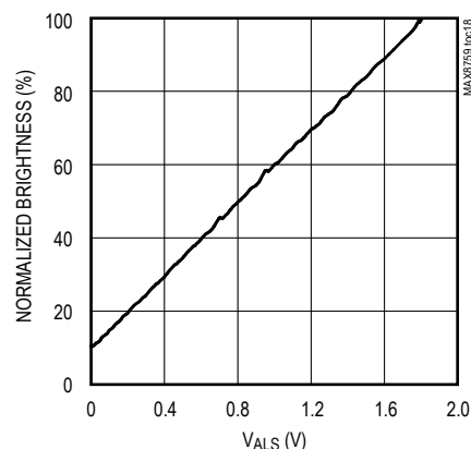
NORMALIZED BRIGHTNESS vs. V_{ALS} VOLTAGE
