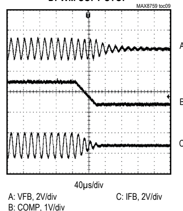
DPWM SOFT-STOP
