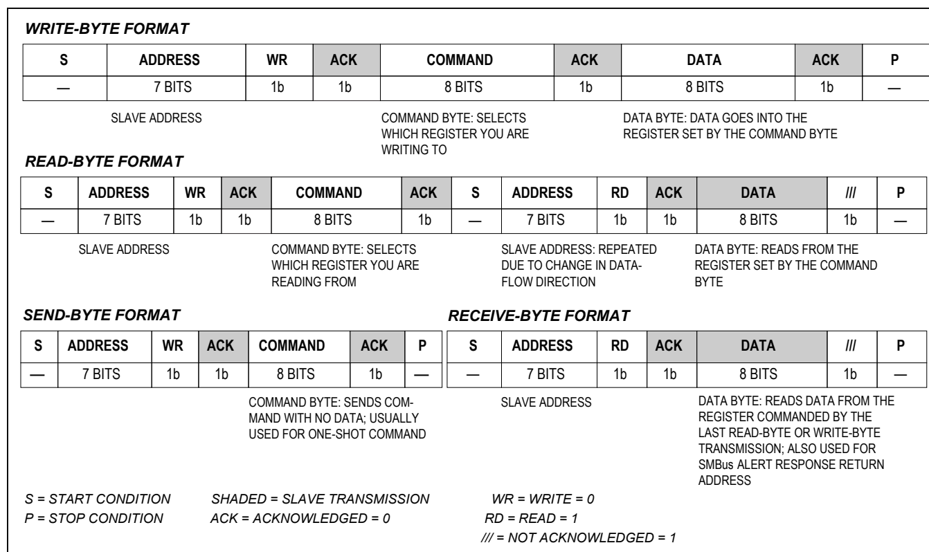
Figure 8. SMBus Protocols
