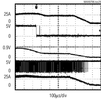
A. LOAD CURRENT, 25A/div B. PGOOD, 5V/div C. V_{OUT} , 1V/div D. DL, 5V/div E. INDUCTOR CURRENT, 25A/div
