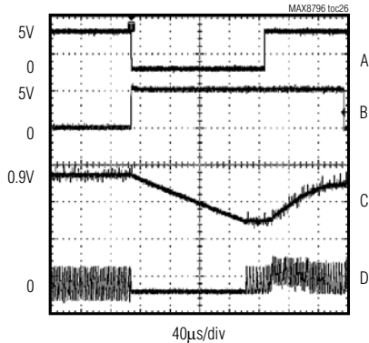
A. \overline{\text{DPRSTP}} , 5V/div B. \text{DPRSLPVR} , 5V/div I_{OUT} = 2\text{A} C. V_{OUT} , 200mV/div D. INDUCTOR CURRENT, 10A/div
