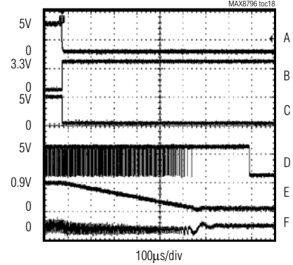
MAX8796/MAX17401 IMVP-6 SHUTDOWN WAVEFORM
