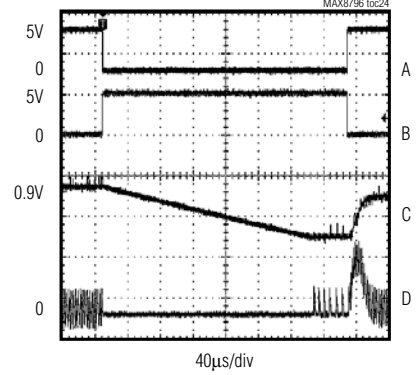
A. \overline{\text{DPRSTP}} , 5V/div B. \text{DPRSLPVR} , 5V/div I_{OUT} = 1\text{A} C. V_{OUT} , 200mV/div D. INDUCTOR CURRENT, 10A/div
