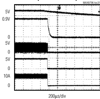
A. 5V BIAS SUPPLY, 5V/div B. V_{OUT} , 500mV/div C. DL, 5V/div D. PGOOD, 5V/div E. INDUCTOR CURRENT, 10A/div
