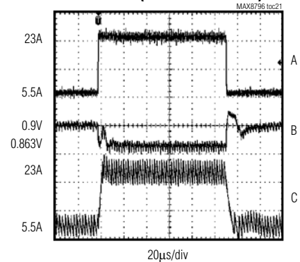
MAX8796/MAX17401 LOAD-TRANSIENT RESPONSE (IMVP-6 HFM MODE)
