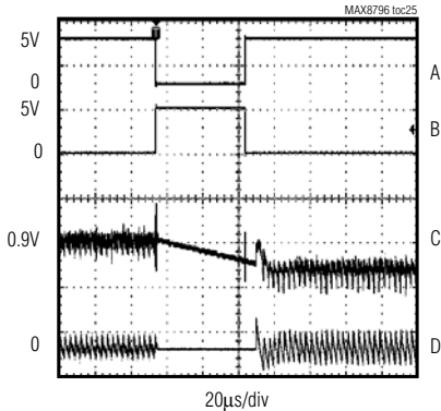
A. \overline{\text{DPRSTP}} , 5V/div B. \text{DPRSLPVR} , 5V/div I_{OUT} = 0.3\text{A} C. V_{OUT} , 20mV/div D. INDUCTOR CURRENT, 10A/div
