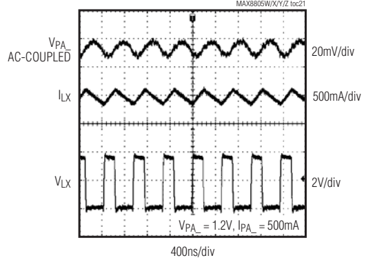
PA STEP-DOWN HEAVY-LOAD SWITCHING WAVEFORMS (MAX8805W/MAX8805Y)
