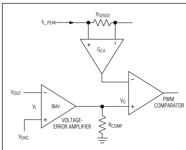
Figure 6. Simplified Peak Current-Mode Control IC with Active Output-Voltage Positioning
