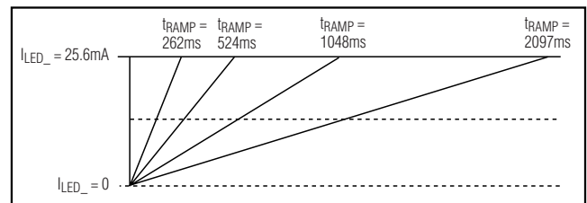
Figure 3. Ramp-Up Behavior
