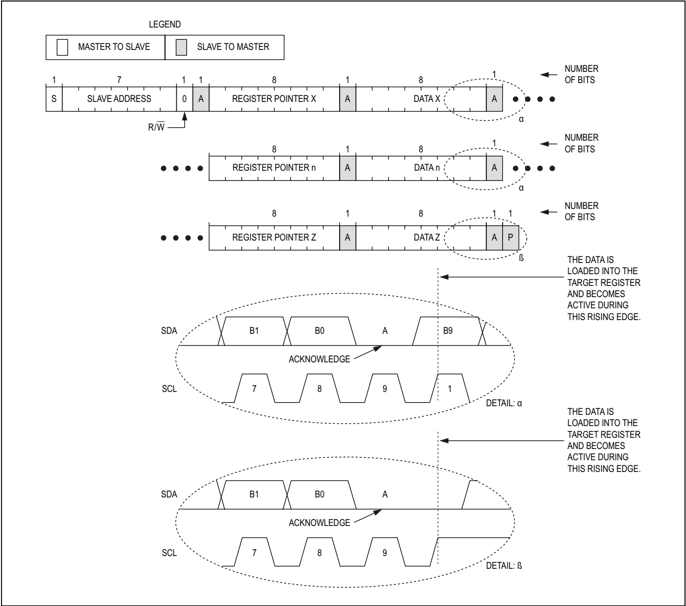
Figure 11. Writing to Multiple Registers with the Multiple Byte Register Data Pair Protocol
