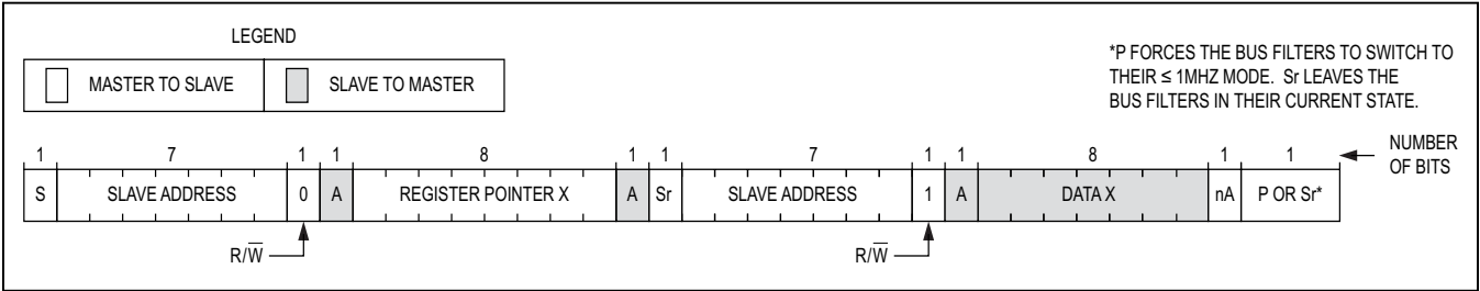
Figure 12. Reading from a Single Register with the Read Byte Protocol
