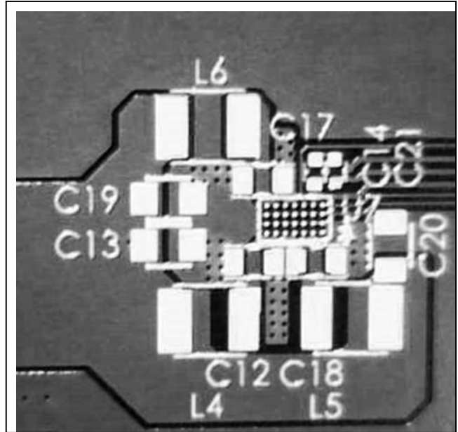
Figure 15. MAX8973_ EVKIT Layout Recommendation
