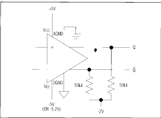
Figure 4a. \pm 5\text{V} Supplies, Separate Ground* * Separate ground is optional. DGND and AGND may be tied together.
