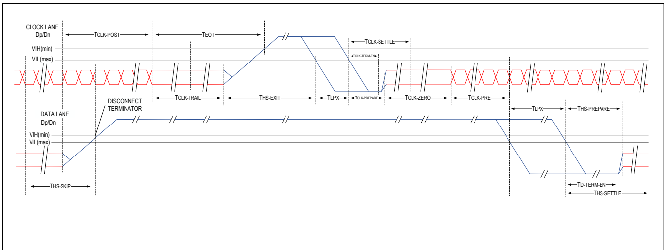
Figure 8. D-PHY Switching Clock Lane From Active Transmission to Low-Power Mode
