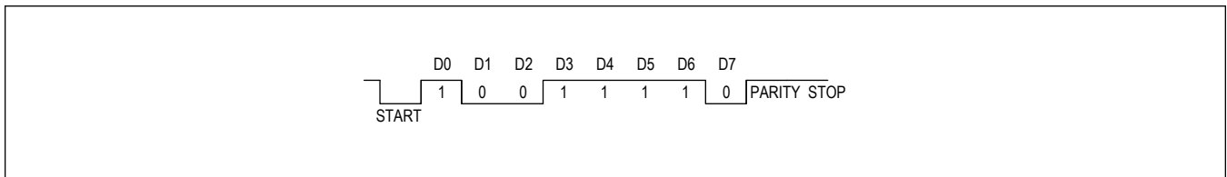
Figure 30. UART Synchronization Frame
