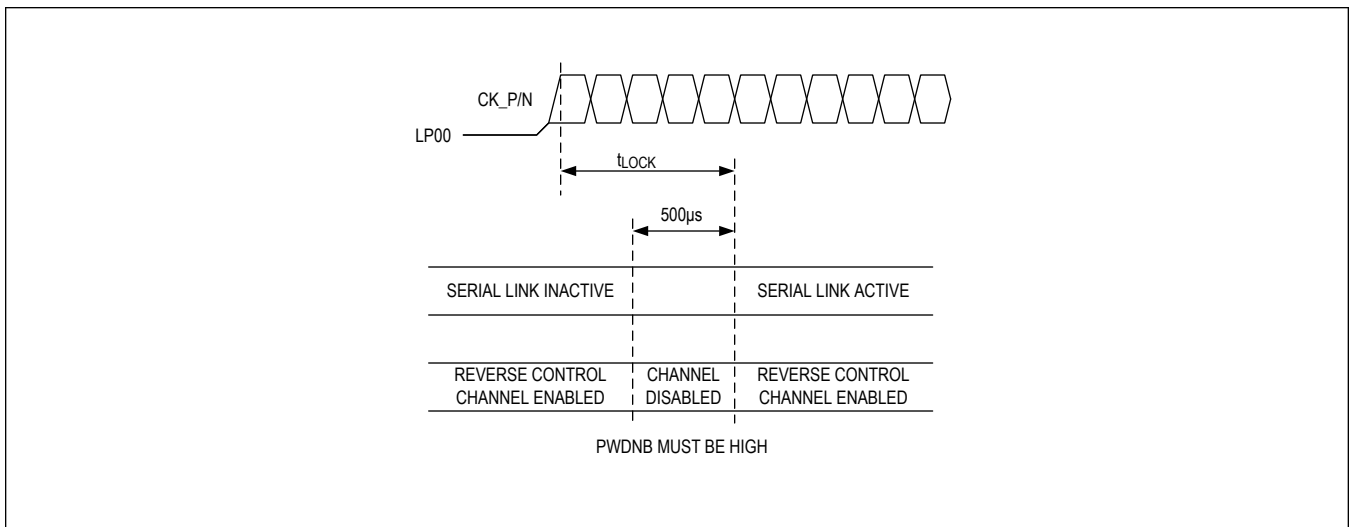
Figure 4. GMSL1 Link Startup Time
