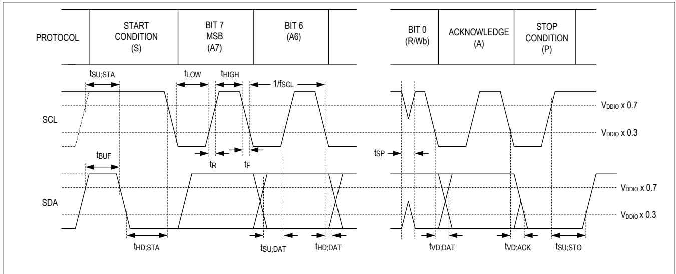
Figure 11. I2C Timing Parameters
