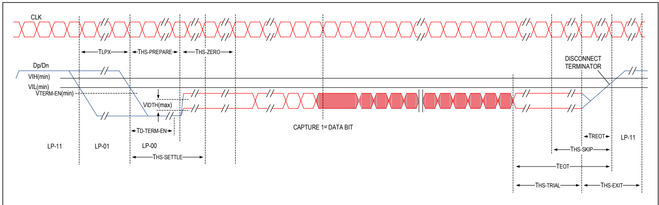
Figure 10. D-PHY HS Burst Data Transmission
