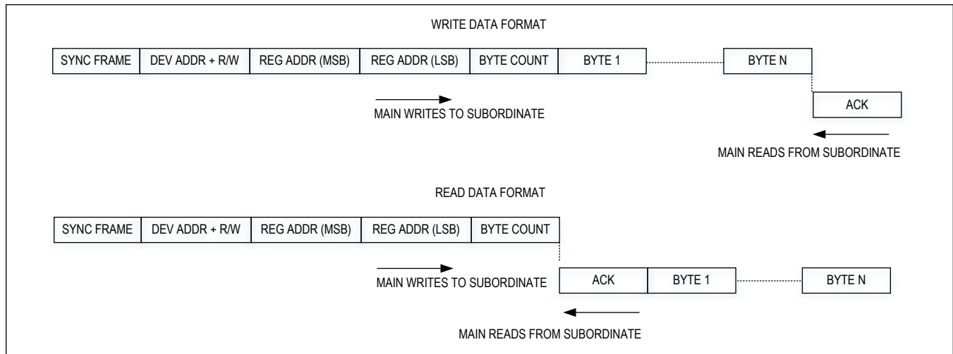
Figure 28. GMSL2 UART Protocol for Base Mode
