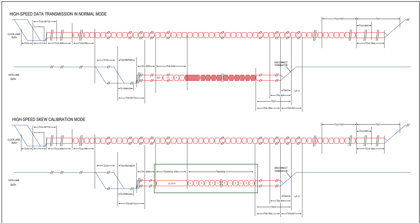
Figure 9. D-PHY Normal Transmission Mode vs Skew Calibration
