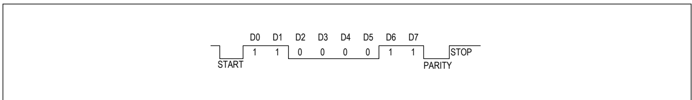
Figure 31. UART Acknowledge Frame
