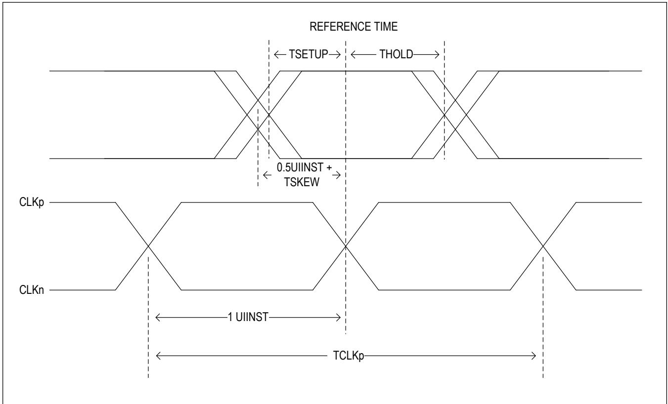
Figure 7. D-PHY Data Clock Timing
