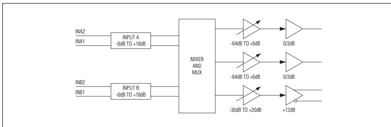
Figure 2. Signal Path
