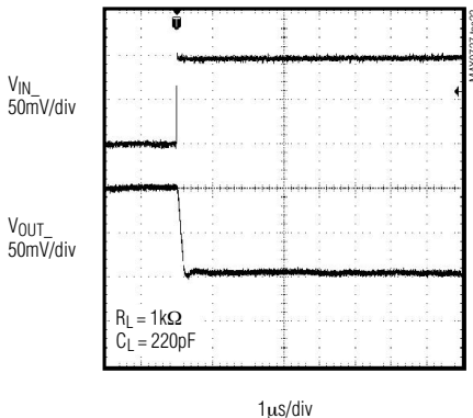
STEP RESPONSE
