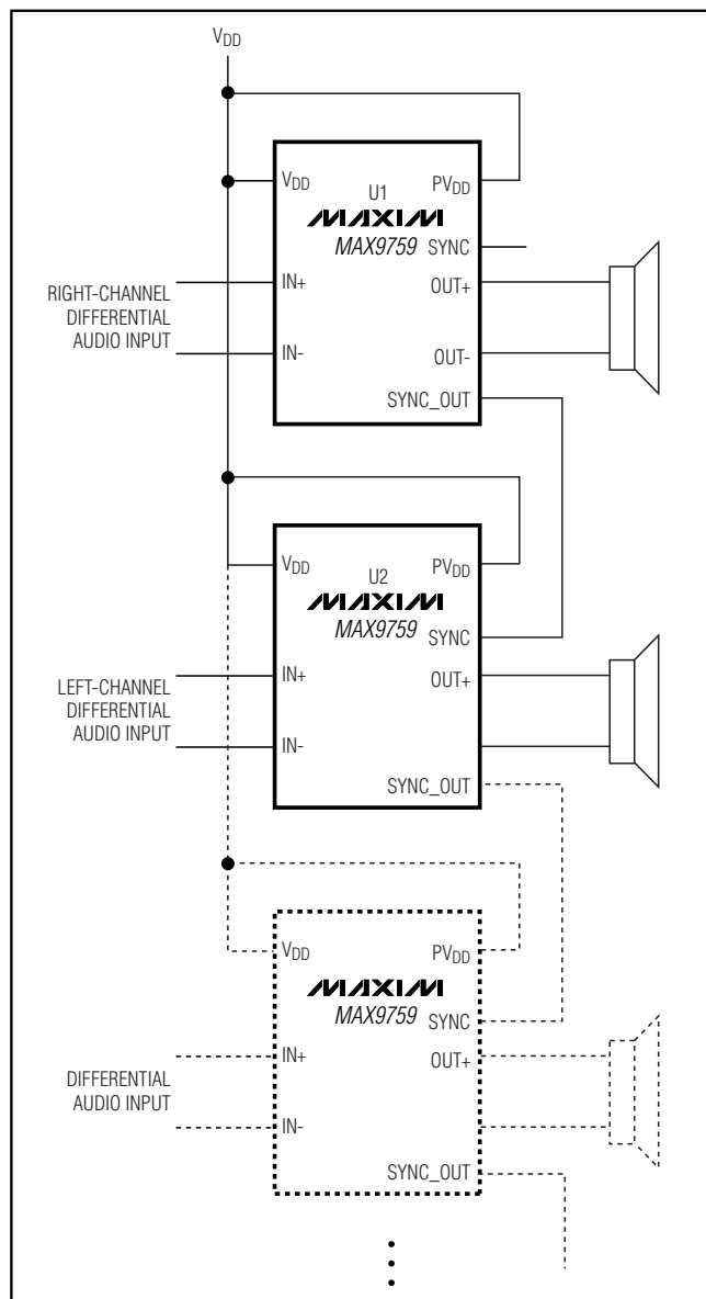
Figure 7. Master-Slave Configuration
