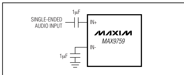
Figure 6. Single-Ended Input
