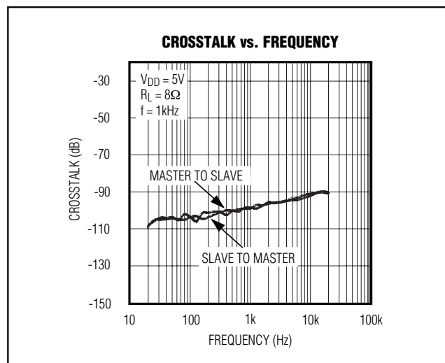
Figure 9. Crosstalk vs. Frequency
