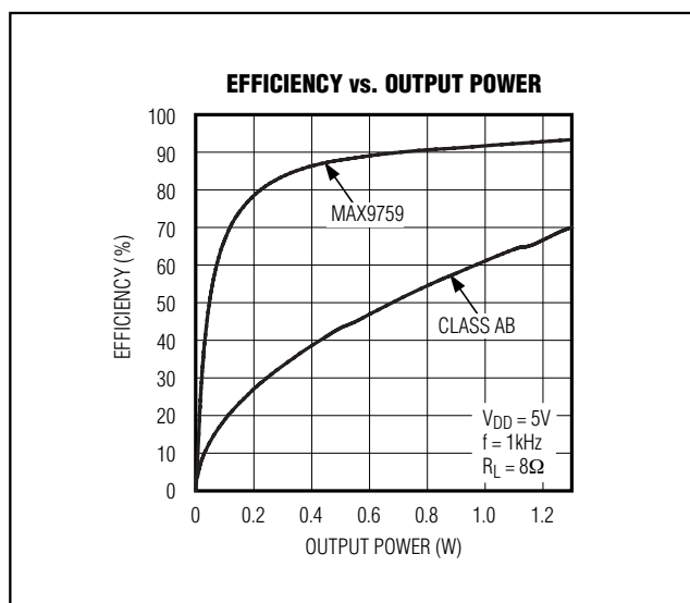
Figure 5. MAX9759 Efficiency vs. Output Power
