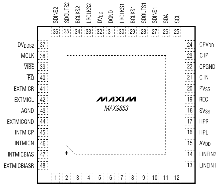
THIN QFN (7mm x 7mm)
