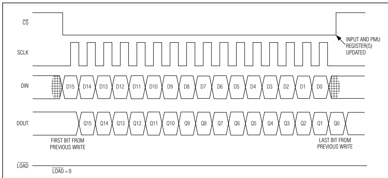
Figure 2. Serial Port Timing with Synchronous Load
