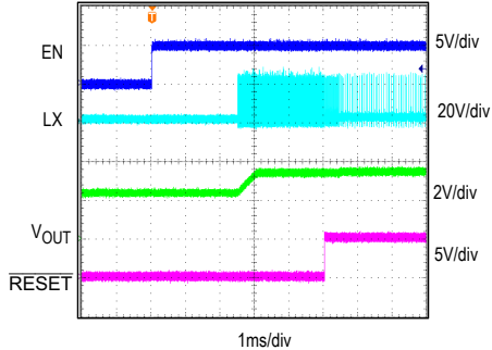
STARTUP WITH 2.5V PREBIAS V_{IN} = 24V, V_{OUT} = 3.3V, I_{OUT} = 0A, MODE = OPEN
