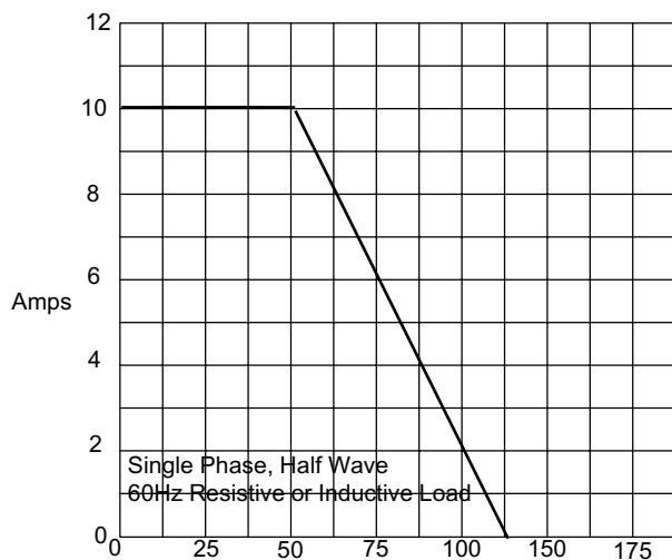
Figure 3 Forward Derating Curve
