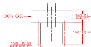
Dimensions in inches and (millimeters)
