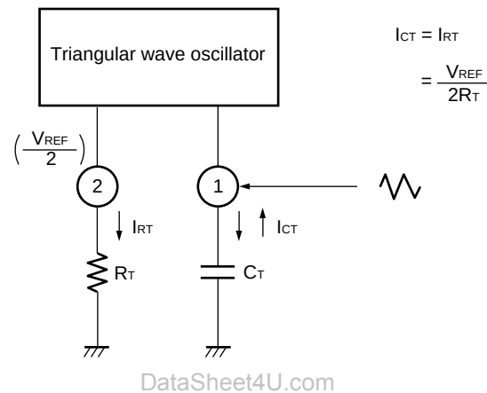
Figure 1 No V_{REF}/2 connection to external circuits from R_T pin
