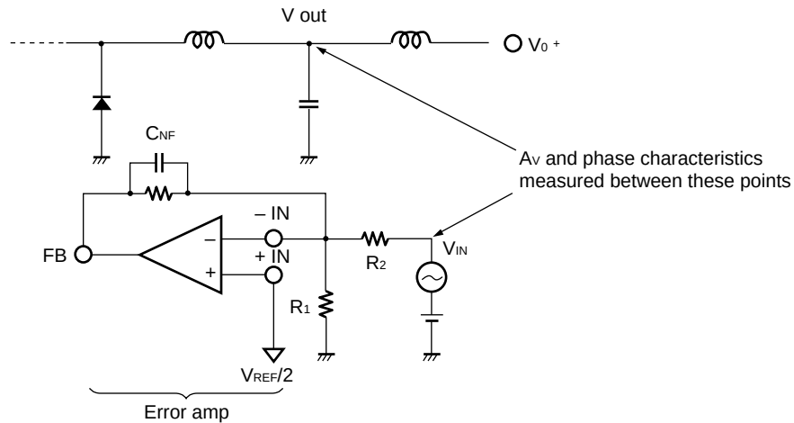
Figure 2 Measurement of DC/DC Capacitor AV and Phase ( \Psi ) Characteristics
