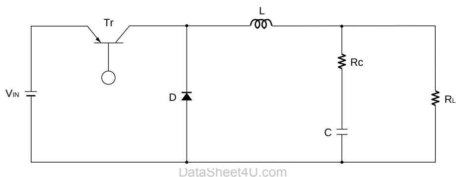
Figure 1 Basic circuit for step-down voltage DC/DC converter
