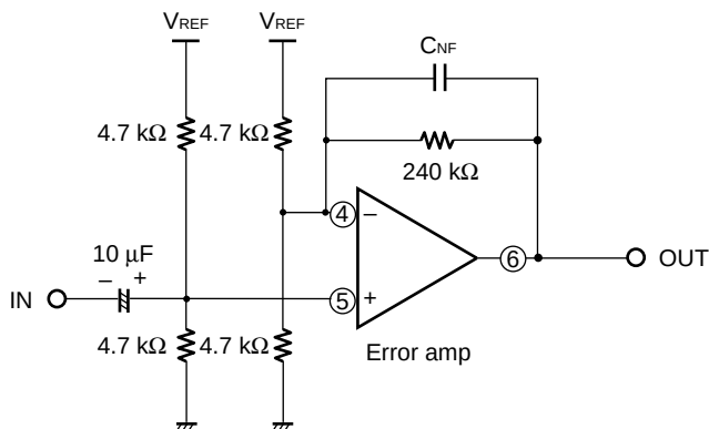
Test Circuit
