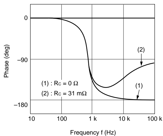
Figure 19. Phase-Frequency Characteristic
