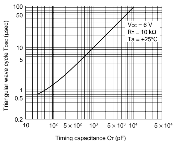
9. Triangular wave cycle vs. Timing capacitance
