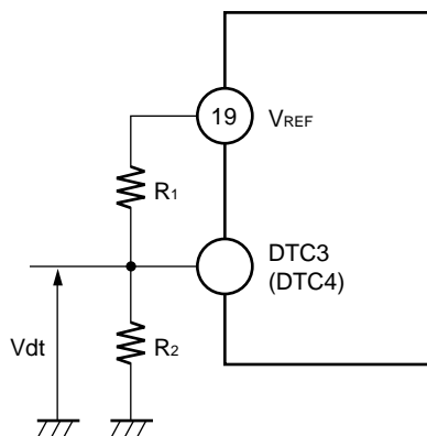
Figure 11. When Using DTC to Set Dead Time
