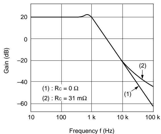
Figure 18. Gain-Frequency Characteristic
