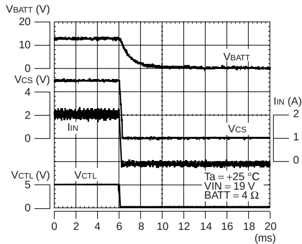
Discharge operating waveform constant current mode (set at 16.8 V)
