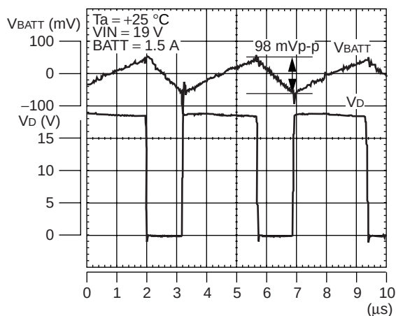
Switching waveform constant voltage mode (set at 12.6 V)
