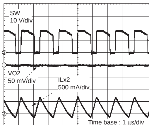
PWM Operation Discontinuous Mode VIN = 12 V, VS = 17.7 V, ILOAD = 10 mA
