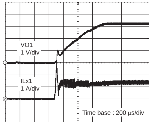
PWM Operation Discontinuous Mode VIN = 12 V, V LOGIC = 3.3 V, I LOAD = 45 mA
