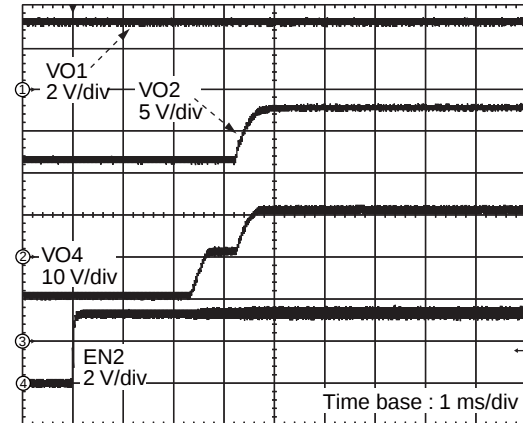
Power-up Sequence EN2 Enabled Separately I Load(VLogic) = 1.5 A, I Load(Vs) = 1.5 A I Load(VGL) = 50 mA, I Load(VGH) = 50 mA
