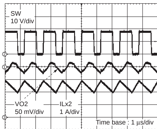
PWM Operation Continuous Mode VIN = 12 V, VS = 17.7 V, ILOAD = 1.5 A
