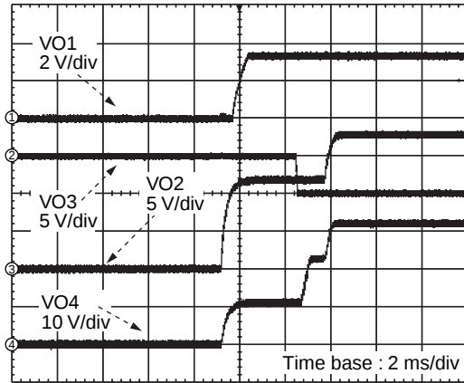
Power-up Sequence VIN = EN1 = EN2 = 12 V All channel without load
