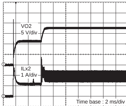
Soft Start VIN = 12 V, VS = 17.7 V, ILOAD = 1.2 A, CSS = 22 nF
