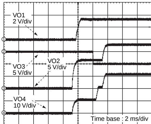
Power-up Sequence VIN = EN1 = EN2 = 12V I Load(VLogic) = 1.5 A, I Load(Vs) = 1.5 A I Load(VGL) = 50 mA, I Load(VGH) = 50 mA
