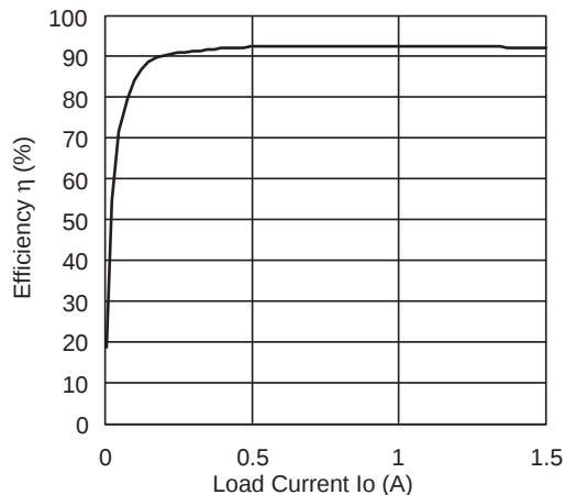
Efficiency vs. Output Current VIN = 12 V, VS = 17.7 V, L2 = 6.8 \mu H
