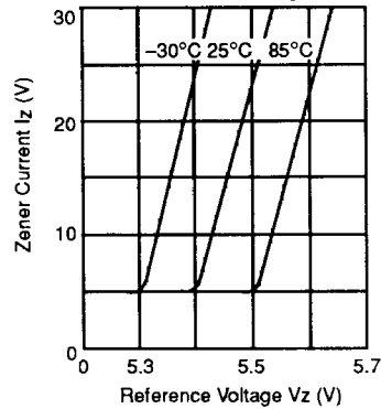
Figure 4. Zener Current vs. Reference Voltage
