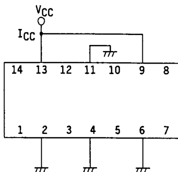
Fig.2 - TEST CIRCUITS
