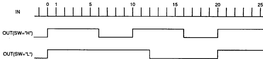
TIMING CHART
