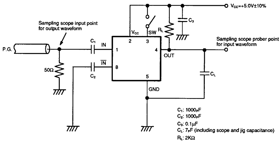
TEST CIRCUIT
