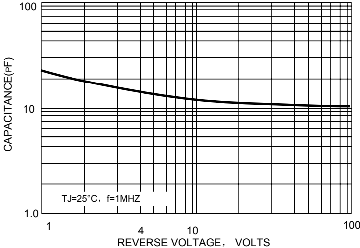
FIG.5-TYPICAL JUNCTION CAPACITANCE
