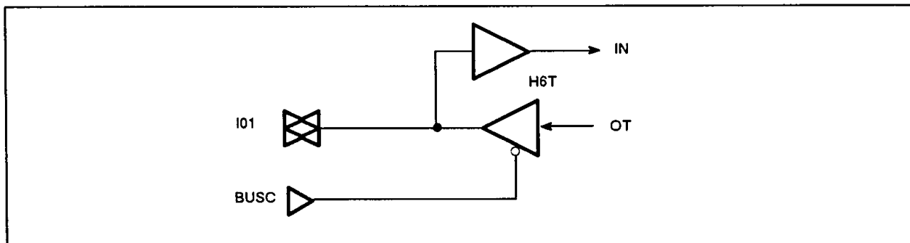
Bidirectional Buffer
