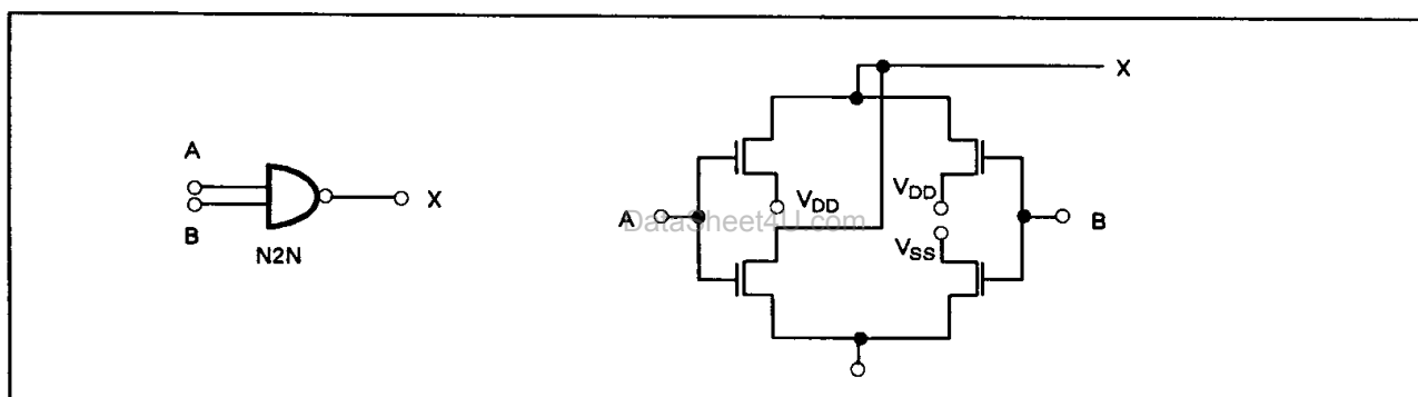
Two-Input NAND Gate Unit Cell (One Basic Cell)
