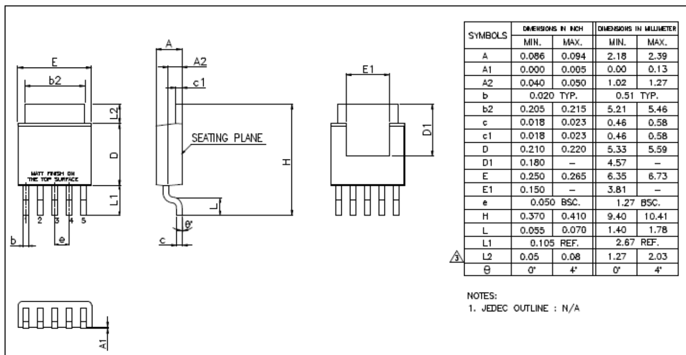
MBI6656 GSD Outline Drawing
