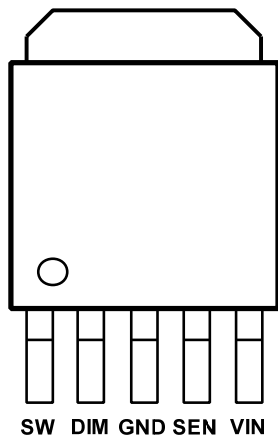
MBI6656GSD (Top View)
