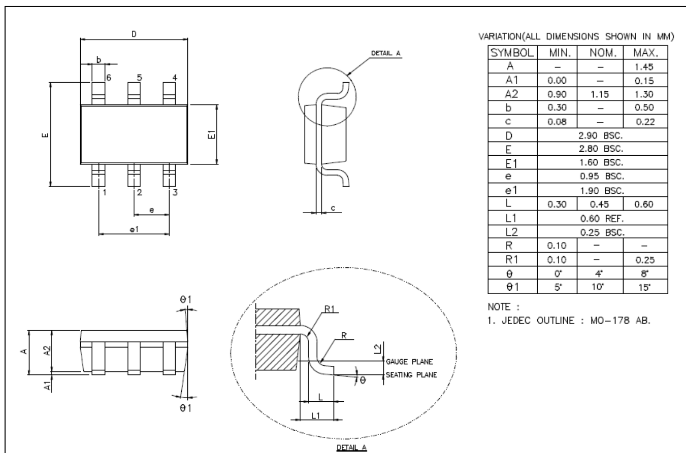
MBI6656 GST Outline Drawing
