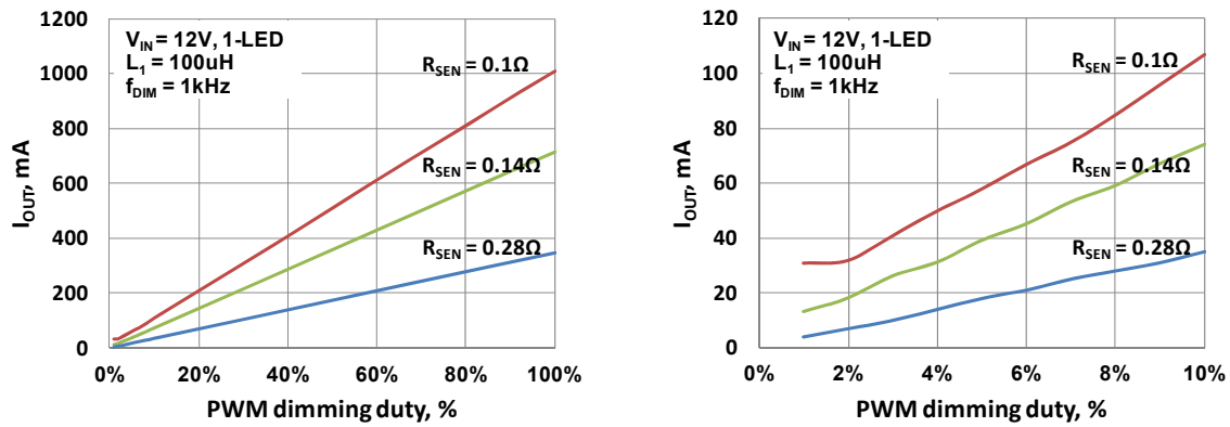
Fig. 15 PWM dimming curve
