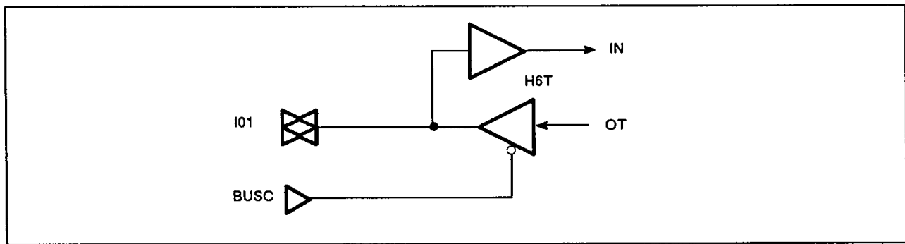
Bidirectional Buffer
