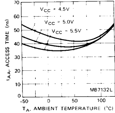
Fig. 13 – t_{AA} ACCESS TIME vs. AMBIENT TEMPERATURE
