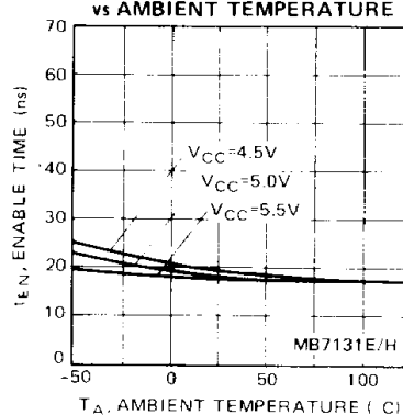
Fig. 18 — t_{EN} ENABLE TIME vs. AMBIENT TEMPERATURE
