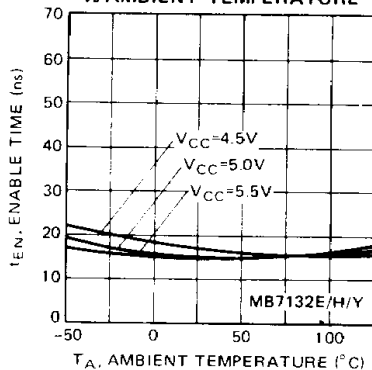
Fig. 19 — t_{EN} ENABLE TIME vs. AMBIENT TEMPERATURE
