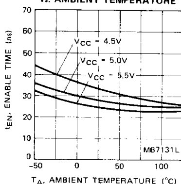
Fig. 20 — t_{EN} ENABLE TIME vs. AMBIENT TEMPERATURE
