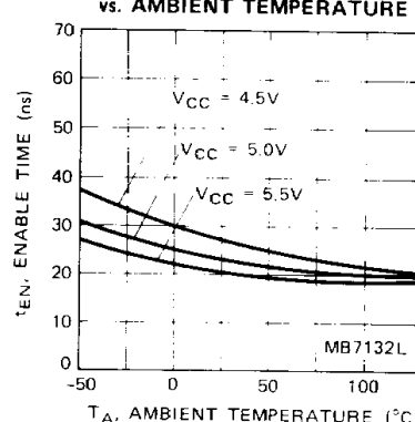
Fig. 21 — t_{EN} ENABLE TIME vs. AMBIENT TEMPERATURE
