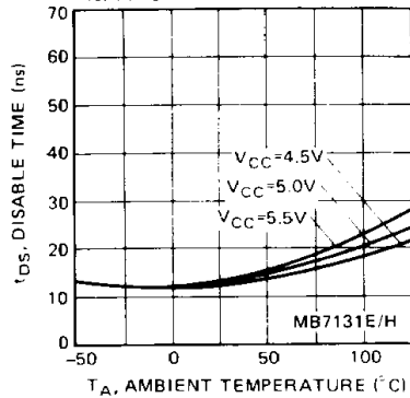
Fig. 14 – t_{DIS} DISABLE TIME vs. AMBIENT TEMPERATURE
