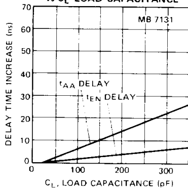
Fig. 22 — DELAY TIME INCREASE vs. C_L LOAD CAPACITANCE
