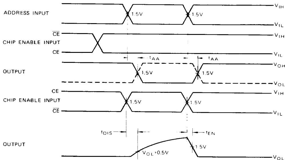
OPERATION TIMING DIAGRAM
