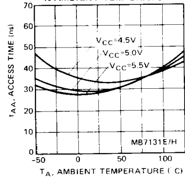
Fig. 10 – t_{AA} ACCESS TIME vs AMBIENT TEMPERATURE
