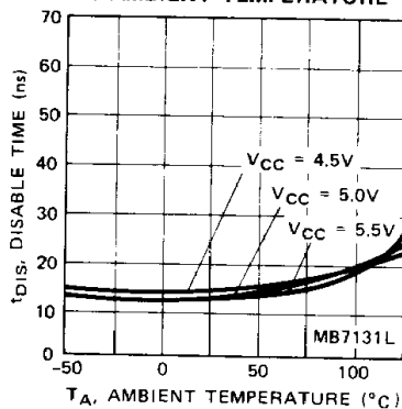
Fig. 16 — t_{DIS} DISABLE TIME vs. AMBIENT TEMPERATURE
