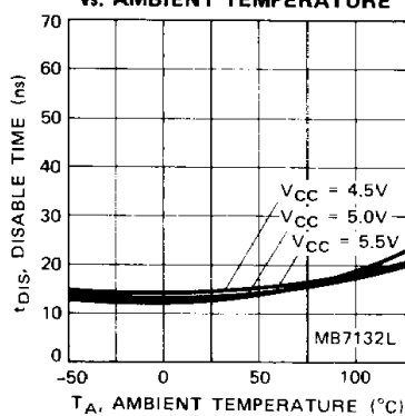
Fig. 17 — t_{DIS} DISABLE TIME vs. AMBIENT TEMPERATURE
