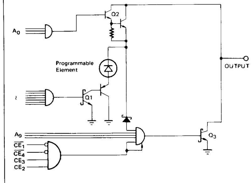
Fig. 25 – INTERNAL PROGRAMMING CIRCUIT
