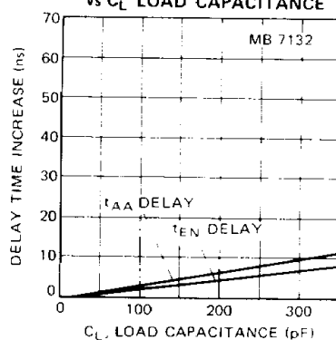
Fig. 23 — DELAY TIME INCREASE vs. C_L LOAD CAPACITANCE
