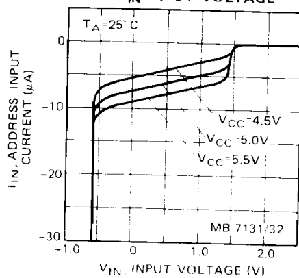
Fig. 6 – I_{IN} INPUT CURRENT vs V_{IN} INPUT VOLTAGE
