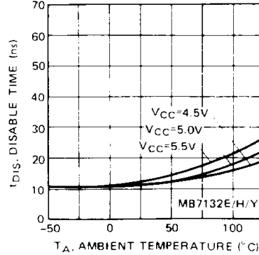
Fig. 15 – t_{DIS} DISABLE TIME vs AMBIENT TEMPERATURE
